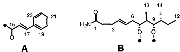
Figure 1. Substructures of basiliskamide A ( 1 ).
